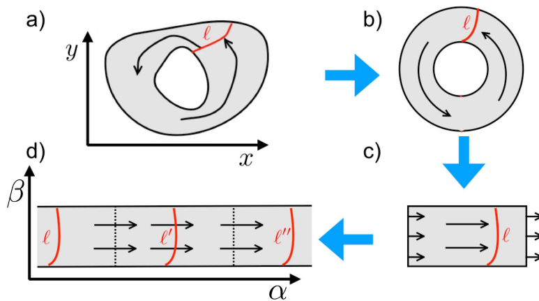
FIG. 2.2. The original ring-like domain (a) (Figure 2.1) is mapped to a true annulus (b), then to the geometric phase and amplitude with periodic boundary conditions (c), and, finally, to a system with unwrapped phase and amplitude (d). In (a), the first return to a simple connection between the two boundaries, l , after one rotation has been performed, is not well defined: we cannot simply turn the line l into an absorbing boundary because then the condition of the performed rotation is not met, and if we start on l , the mean-return-time will be zero. In the unwrapped phase and amplitude (d), we deal with infinitely many concatenated copies of the system, and thus the return-time problem is now well posed: it is given by the first passage problem between two adjacent copies of the line (e.g., from l to l' or from l' to l'' ).
