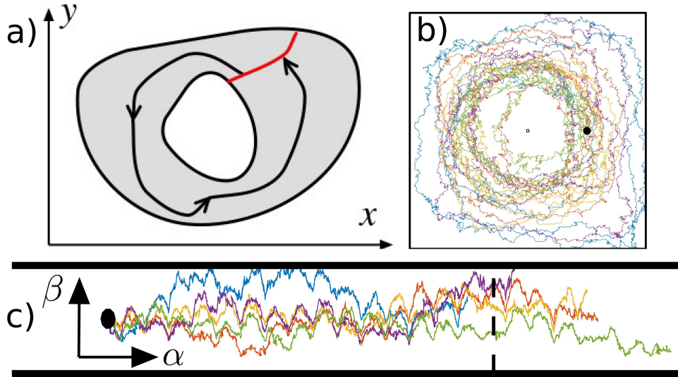
FIG. 2.1. Original ring-like domain with a counterclockwise net probability flow and reflecting inner and outer boundaries (a). An isochron (sketched in red) can be defined by the property that the mean–return-time from any point of this line to itself (after one complete rotation) is given by the overall mean rotation time of the stochastic oscillator. Five trajectories of the noisy heteroclinic oscillator, (4.5), on the original domain (b) and in unwrapped coordinates (c). The common initial condition is marked with a black dot. The inner boundary of the annulus (b) is the square \max(|x|, |y|) = \epsilon = 0.05 , which is mapped to the lower edge of the unwrapped domain, \beta = -1 . The outer boundary of the annulus is mapped to the upper edge of the unwrapped domain, \beta = +1 . The transformation maps point (x, y) to (\alpha, \beta) such that \tan(\alpha) = y/x , with \alpha continuous along trajectories. For the quarter wedge x \geq |y| of the annular domain, we set \beta = -1 + 2(x - \epsilon)/(\frac{\pi}{2} - \epsilon) . In the other quarter wedges of the annular domain, \beta is determined by a similar construction. The vertical dashed line marks one full rotation from the initial point. Compare with Figure 4.5. (Color available online.)
