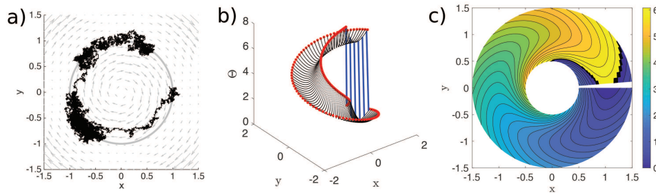
FIG. 4.2. Stuart–Landau oscillator with antirotating phase , (4.3), with \omega = 1 , \gamma = 15 , c = -15 , and D = 0.198 . Sample trajectory ( \Delta t = 10^{-4} ) for an initial condition at (1, 0) , limit cycle (grey bold line) and vector field shown by arrows (a), MRT phase \Theta(x, y) from the finite-difference-scheme solution (b), and its contour lines, i.e., the isochrons of the MRT phase (c). For the parameters used, \bar{T} = 11.89 .
