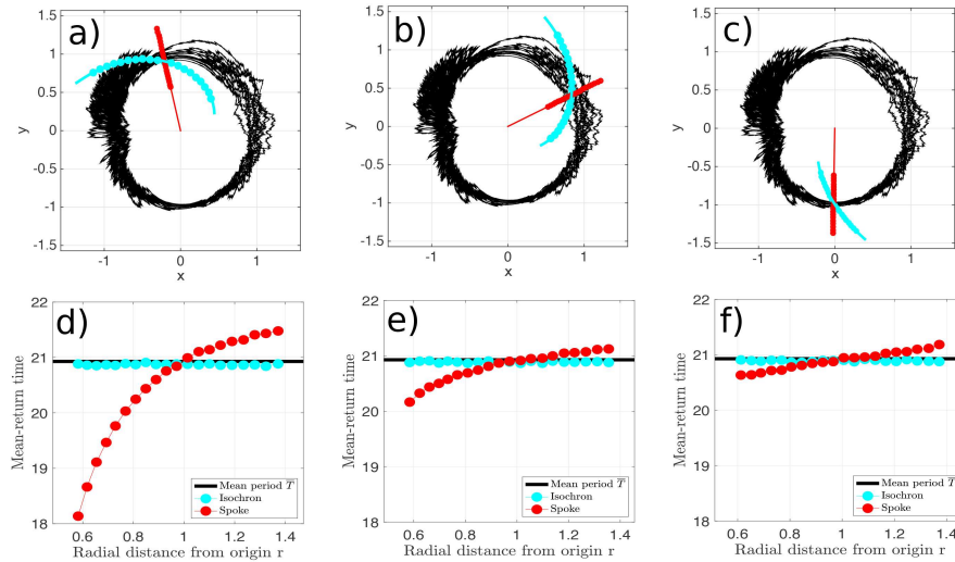
FIG. 4.4. Testing the MRT property for the noisy Stuart-Landau oscillator with y -polarized noise (4.4). Sample trajectory ((a)–(c), black trace) and parameters are as in Figure 4.3. Cyan curves (a)–(c) show isochronal sections obtained from the PDE solution; red curves are “spoke” sections passing through the isochronal section. For each of 20 points per curve, equally spaced in the radial coordinate, we generate approximately 600,000 independent trajectories, using the Euler-Maruyama method (trajectories generated in polar (r, \theta) coordinates with \Delta t = 0.001 ) and computing the MRT from a starting point to the same section after completing one rotation (d)–(f). For initial conditions on the PDE-derived isochrons, mean-return-times ((d)–(f), cyan dots), are within 0.5% of the mean period ((d)–(f), black horizontal line). For initial conditions on a spoke, MRTs deviate significantly from the mean period ((d)–(f), red dots). Thus the isochronal sections obtained as level curves of T(x, y) solved with the periodic-plus-jump condition are an MRT isochron in the sense of S&P, whereas the spoke shows a strong increase of the mean-return-time with growing radius and is thus not such an isochron. (Color available online.)
