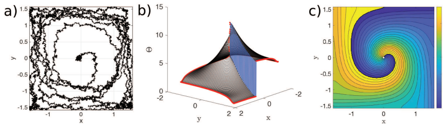
FIG. 4.5. Noisy heteroclinic oscillator , (4.5), with \alpha = 0.1 and D = 0.01125 . Sample trajectory ( \Delta t = 0.001 ) with initial condition at (0, 0) that moves clockwise (a). In the absence of noise, the system has a stable heteroclinic orbit with infinite period. With noise ( D > 0 ), the small perturbations eventually knock the trajectory out of the corners to form a stochastic oscillator with finite mean period. MRT phase \Theta(x, y) finite-difference-scheme solution (b) and its contour lines, i.e., the isochrons of the MRT phase (c). The computational grid is 251 \times 251 and the punctured square has side length of 0.05. For the parameters used, \bar{T} = 16.23 .
