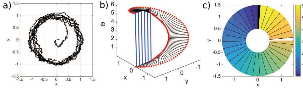
FIG. 4.1. Isochronal Stuart-Landau oscillator clock model, (4.1), with \omega = 1 , \gamma = 1 , and D = 0.01 . Sample trajectory (with timestep \Delta t = 0.001 ) with initial condition at (0,0) (a), MRT phase \Theta(x,y) obtained by a finite difference scheme (b), and its contour lines (c), which are the MRT isochrons. As expected, the isochrons are spokes of the wheel, and each “spoke” is constant up to the order of 10^{-12} . For the parameters used, \bar{T} = 2\pi .
