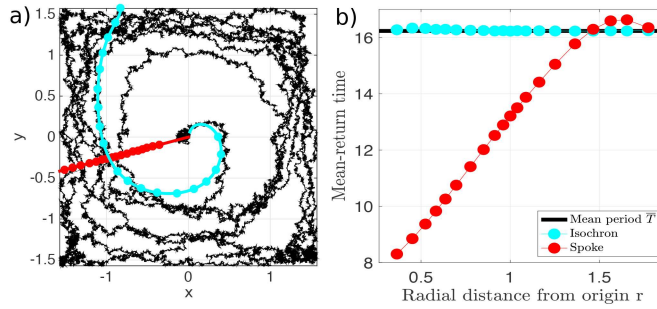
FIG. 4.6. (a) Heteroclinic trajectory in black for D = 0.01125 and \alpha = 0.1 with initial condition at origin. The cyan curve is an isophase pulled from the contour plot in Figure 4.5(c). The cyan dots indicate 20 equally spaced initial conditions along this curve. The red curve is a “spoke” running through the tenth isophase initial condition. The red dots indicate 20 equally spaced initial conditions. (b) The black line is the mean period calculated from the stationary flux (used in the finite difference scheme). Cyan dots are the MRTs back to the isophase after completing one full oscillation of the isophase initial conditions, from an ensemble of approximately 520,000 trajectories generated using the Euler–Maruyama method with \Delta t = 0.001 . The x-axis is the radial distance from the origin. Red dots are the MRTs back to the spoke after completing one full rotation from the spoke initial conditions. (Color available online.)
