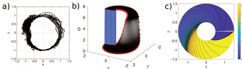
FIG. 4.3. Noisy Stuart–Landau oscillator with y -polarized noise given by (4.4) with \omega = 1.99 , \kappa = 1 , and \sigma = 0.2 . Example trajectory (a) ( \Delta t = 0.01 , trajectories generated in polar (r, \theta) coordinates and then converted to Cartesian (x, y) for analysis), MRT phase \Theta(x, y) (b), and its contour lines, i.e., isochrons of the MRT phase (c). For the parameters used, \bar{T} = 20.93 .
