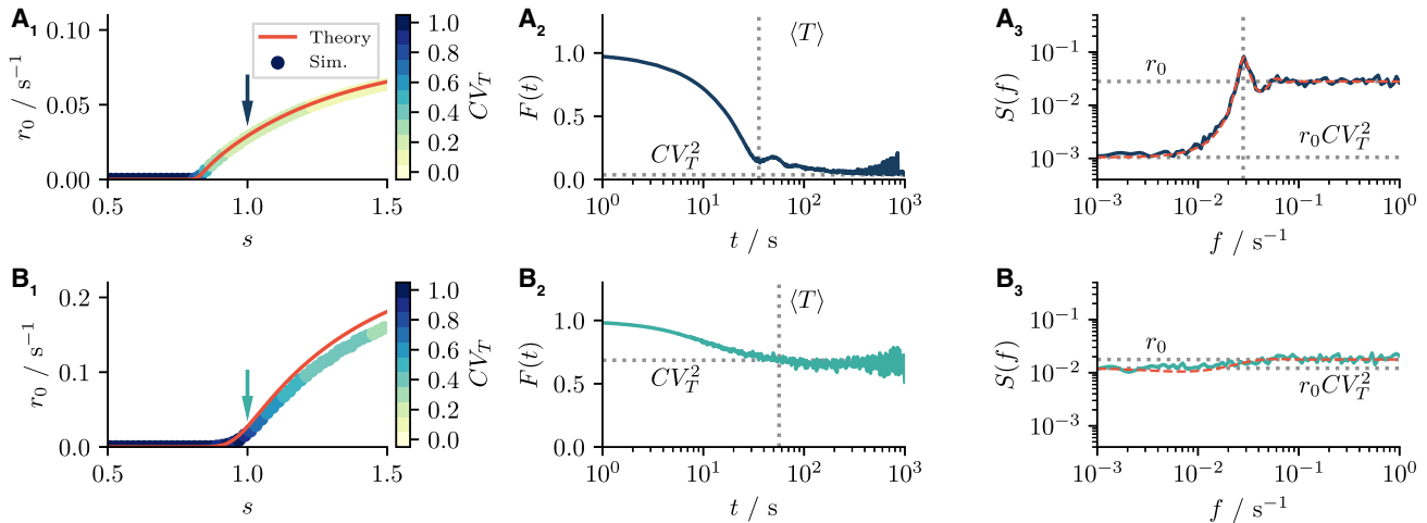
FIGURE 7 Spike-train statistics in the mean-driven and excitable regime. (A and B) The model is in the mean-driven and excitable regime, respectively. ( A_1 and B_1 ) Show the firing rate r_0 = 1/\langle T \rangle obtained from simulations of the two-component model (circles) and theoretical prediction according to Eq. 62 (red line) both as a function of the relative \text{IP}_3 concentration s . The dots are colored coded according to the CV_T . Arrows indicate the value of s that has been used in the previous figures and is used for the remaining plots. ( A_2 and B_2 ) Show the Fano factor that compares the variance to the mean of the spike count. Horizontal dotted lines indicate the long-time limit F(t \rightarrow \infty) = CV_T^2 that is approached if the spike train is renewal. Vertical lines indicate the mean ISI \langle T \rangle that defines a characteristic time up to which the Fano factor decreases almost linearly (difficult to see in the lin-log presentation of the plot). ( A_3 and B_3 ) Depict the power spectrum directly computed from the simulated spike train (blue lines) and from Eq. 41 using an inverse Gaussian distribution according to Eq. 42 (dashed red line). Horizontal lines indicate the low frequency limit of a renewal spike train S(f = 0) = r_0 CV_T^2 and high frequency limit S(f \rightarrow \infty) = r_0 . Parameters: K = 10 , (A): \tau = 5 , p = 1.5 \times 10^{-2} , (B): \tau = 1 , p = 6 \times 10^{-2} . To see this figure in color, go online.
