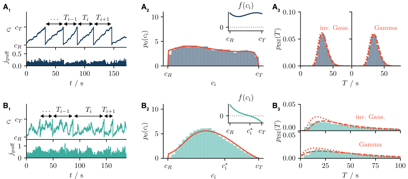
FIGURE 5 Two-component model in the mean-driven and excitable regime. ( A and B ) The model is in the mean-driven and excitable regime, respectively. ( A 1 and B 1 ) Show the subthreshold dynamics of c_i and the puff current j_{\text{puff}} . Already with the naked eye it can be seen that the corresponding ISI sequence marked by black arrows is more regular in ( A 1 ) than in ( B 1 ). ( A 2 and B 2 ) We compare the corresponding subthreshold probability densities p_0(c_i) obtained from stochastic simulations of the two-component model ( histograms ) to the theoretical prediction according to Eq. 61 ( red lines ). The insets in ( A 2 ) and ( B 2 ) shows the drift f(c_i) that is always positive in the mean-driven regime ( A 2 ) but exhibits a zero at c_i^* in the excitable regime ( B 2 ). ( A 3 and B 3 ) The ISI densities determined from numerical simulations ( histograms ) are compared with inverse Gaussian and gamma distributions ( red lines ) as indicated by the red text. Both distributions are uniquely determined by the mean \langle T \rangle and CV CV_T that have been taken either directly from stochastic simulations of the two-component model ( dashed red lines ) or calculated according to Eq. 62 and Eq. 69 ( dotted red lines ). In the mean-driven regime all four variants are in excellent agreement with the ISI density obtained from the two-component model. In the excitable regime the inverse Gaussian provides a better estimate than the gamma distribution to the ISI density obtained from stochastic simulations of the two-component model. In addition, mean and CV obtained from the two-component model and the Langevin approximation begin to differ so that the distributions ( dashed and dotted red lines ) disagree. Parameters: K = 10 , ( A ): \tau = 5 , p = 1.5 \times 10^{-2} , ( B ): \tau = 1 , p = 6 \times 10^{-2} . To see this figure in color, go online.
