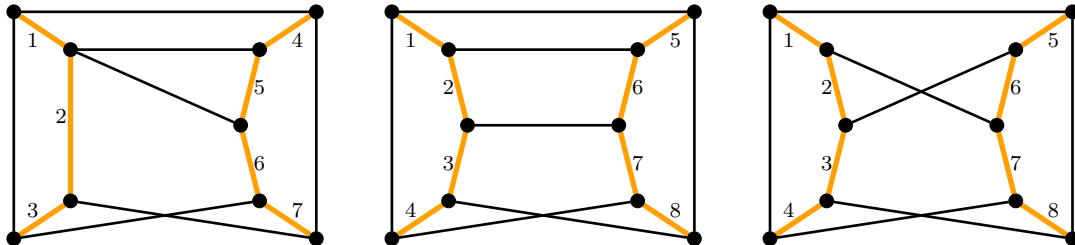
Figure 7: An element of the sum Z_n with its two possible pre-images under \partial_C .
