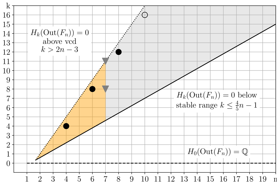
Figure 6: Homology classes of \text{Out}(F_n) . The circles represent the Morita classes and are filled in if they are known to be non-trivial. The triangles are Bartholdi's non-trivial classes. The orange shaded region represents the area where the homology is known to be trivial. The grey shaded area is the unknown homology.
