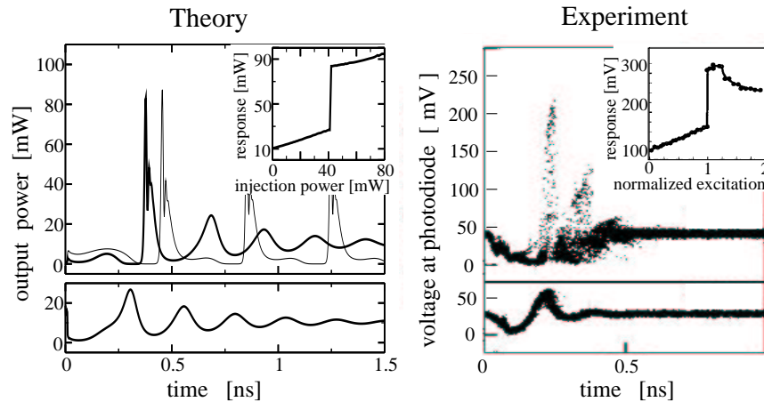
Figure 4. Left: theoretical predictions. Right: experimental results. Upper and lower diagrams show response of the laser due to super- and sub-threshold perturbation. Thin and thick lines in the upper left diagram are due to perturbation of stationary state at different phase conditions. Sampling technique was used drawing experimental diagrams. The inserts show nonlinear response function of laser due to perturbations of different strength.
