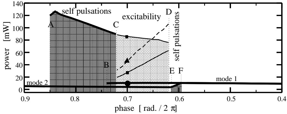
Figure 3. Solid thick lines show stable stationary solutions or maximal value of stable self pulsating solution. Thin solid and dashed lines show strength of threshold injection and response of the system just before and after threshold perturbation. Intensively and light shadowed areas indicate regions where stable self pulsations and excitability can be observed, respectively.
