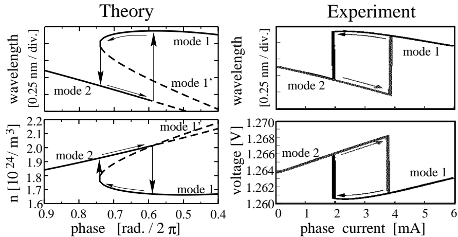
Figure 2. Left: theoretical predictions. Right: experimental results. Solid and dashed thick lines show stable and unstable stationary solutions. Upper diagrams: lasing wavelengths of the stationary states. Lower diagrams: threshold carrier density (theory) and applied voltage (experiments). Bistability is observed in the interval [B, F] .
