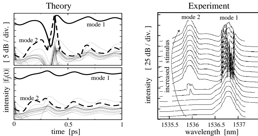
Figure 5. Left: theoretical results. Evolution of the mode decomposition coefficients |f_j(t)| when approaching stable stationary state after super-threshold (above) and sub-threshold (below) perturbation. Thick lines represent coefficients of two modes which have the main impact in the super-threshold perturbation case. Right: experimental results. A sequence of measured optical spectra for different power of injected pulse. An influence of two modes are visible in the super-threshold perturbation case.
