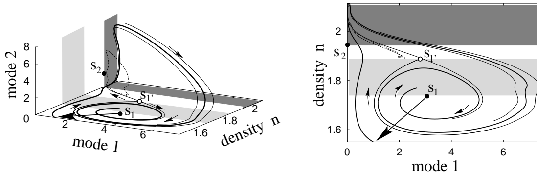
Figure 6: Projections of the phase space of the excitable system at \varphi = 0.7 onto three- or two-dimensional subspace.
