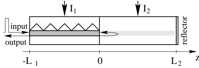
Figure 1: Scheme of a DFB laser with integrated short external cavity.
